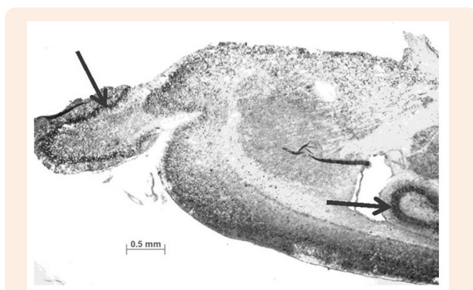
Figure 1: In situ hybridisation with nrp gene specific anti-sense cRNA probe when incubating it with sagittally processed P0 mouse brain slices is showing nrp expression in the olfactory mitral cell layer as well as hippocampal CA1/CA3 expression (arrows are indicating the nrp-positive regions). The cRNA probe is highly specific and results in no signal when being tested as sense probe. The probe consists of a nucleotide sequence (88-mer) deriving from the transcription start region of the mouse nrp gene.
